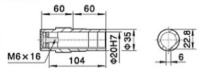
SAF37/SA37/SAZ37 空心轴/Hollow shaft
