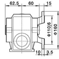
SAF37/SA37/SAZ37 空心轴/Hollow shaft
