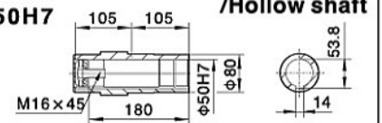
SA77/SAZ77/SAF77空心轴
