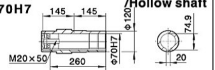
SA97/SAZ97/SAF97空心轴
