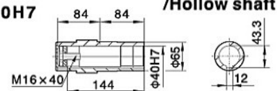
SA67/SAZ67/SAF67空心轴
