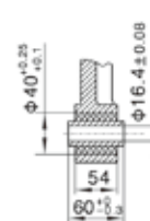
D side of torque-arm
