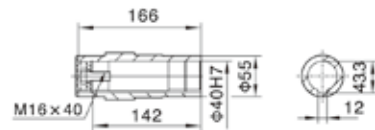
FA57/FAF57/FAZ57 /Hollow shaft
